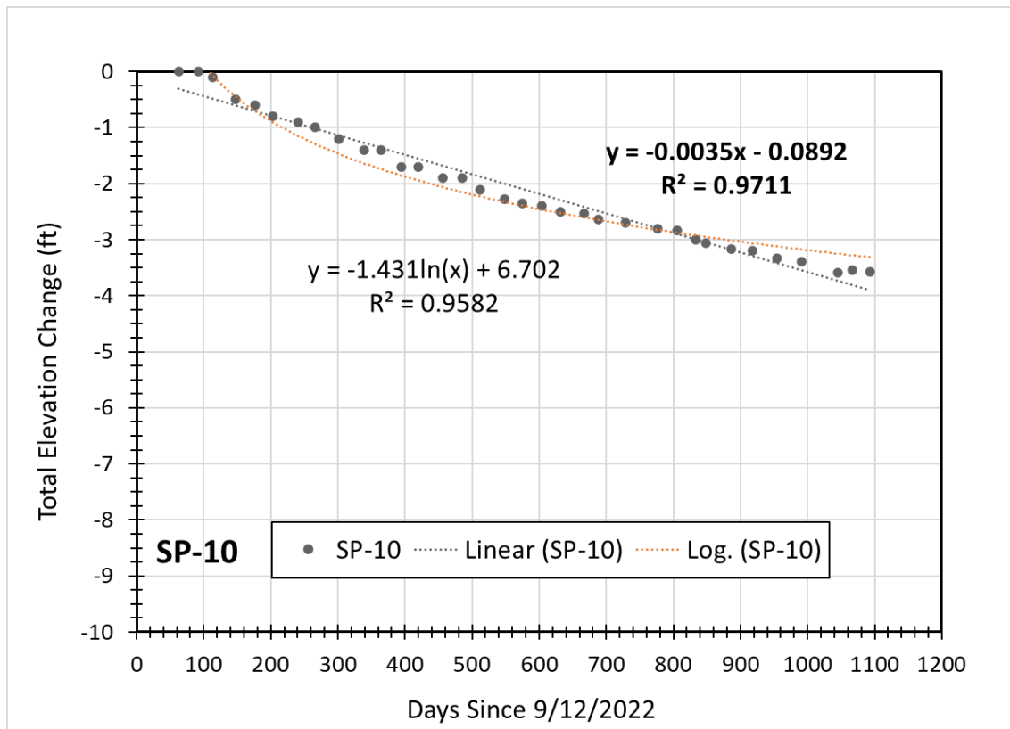
Figure 11 - Settlement Plate SP-10
