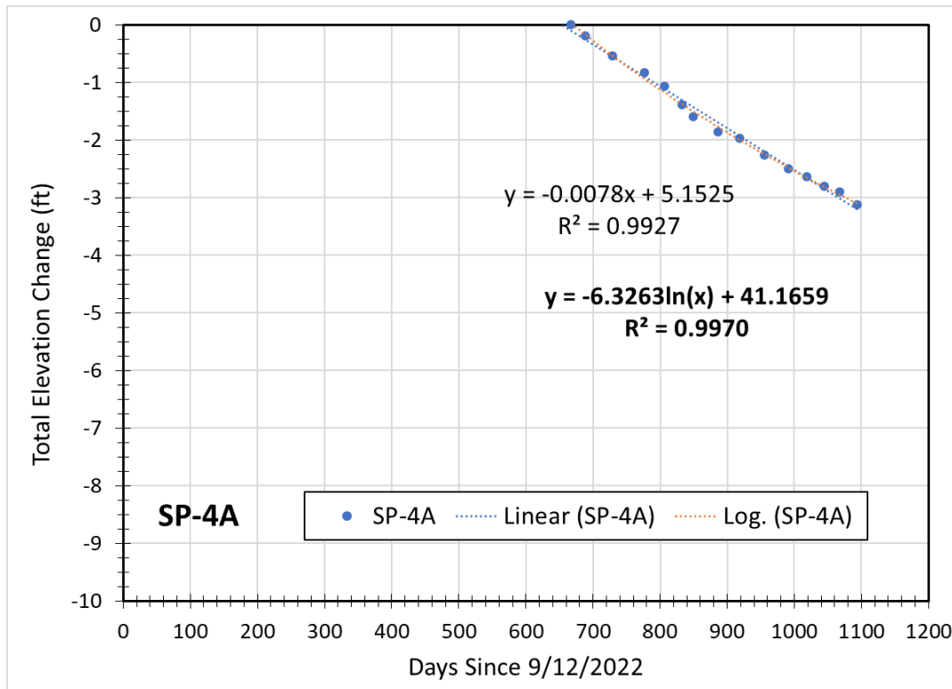
Figure 5 - Settlement Plate SP-4A
