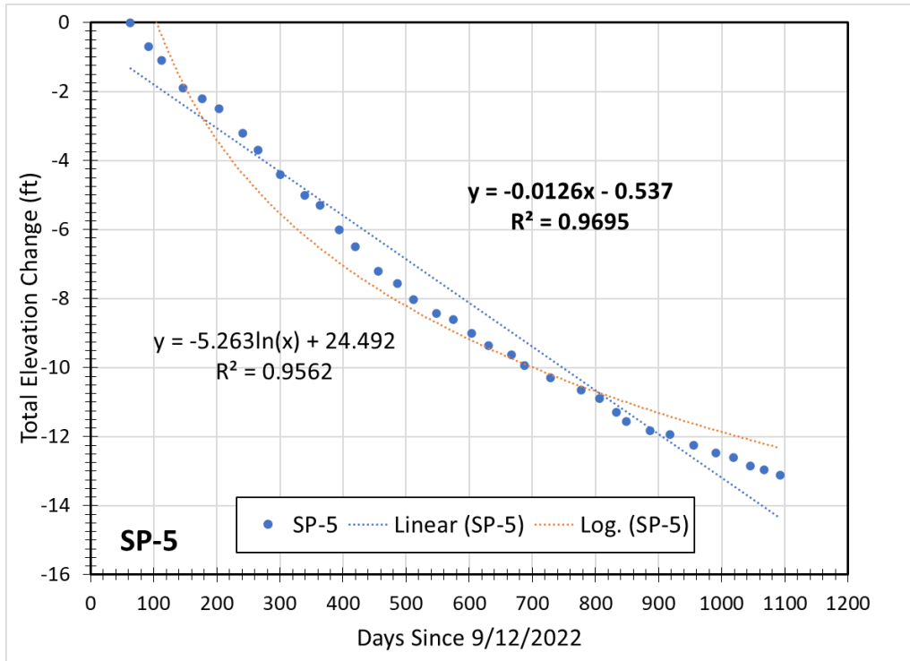
Figure 6 - Settlement Plate SP-5
