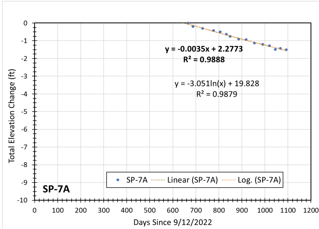
Figure 8 - Settlement Plate SP-7A
